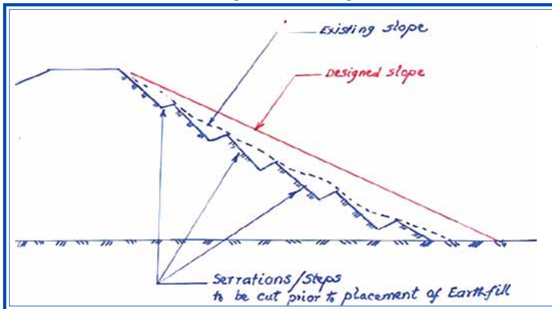
FIG:2 INDICATING SERRATIONS
