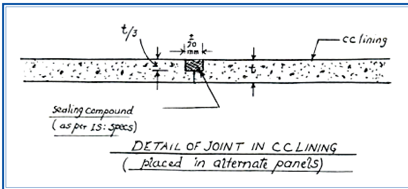
FIG: 18 JOINT IN CC LINING
